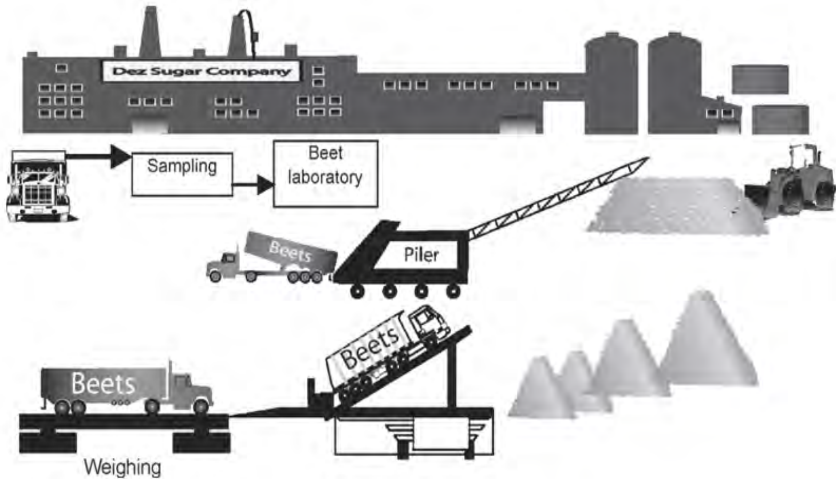
Figure 3.1.1 Flow diagram of beet receiving and storage (Station 1)
